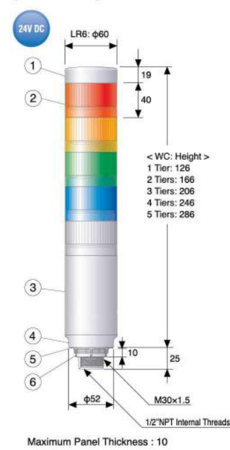
[WC] Direct Mount with M12 Connector (02: 24V DC)
